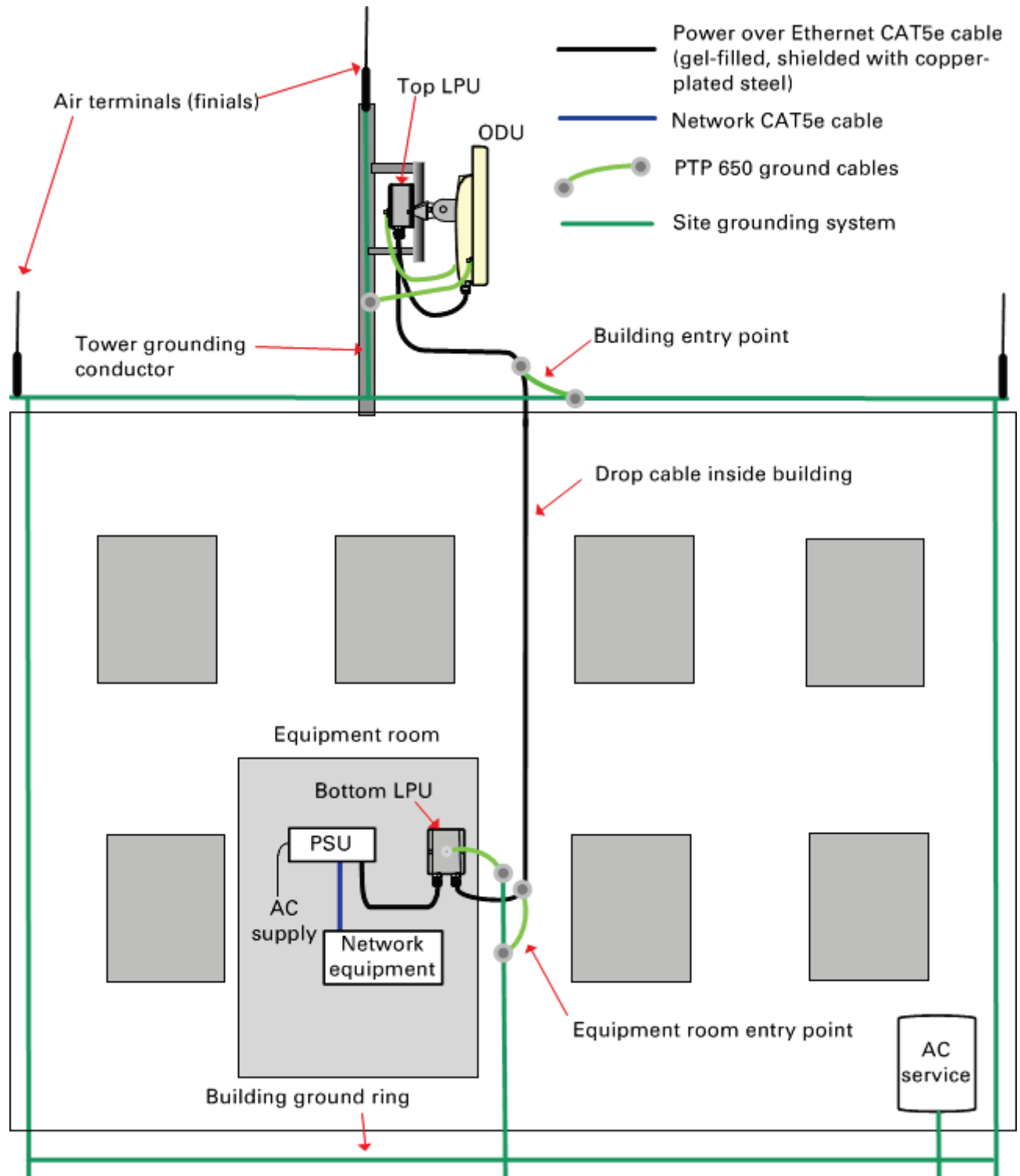
Figure 35 Roof installation
