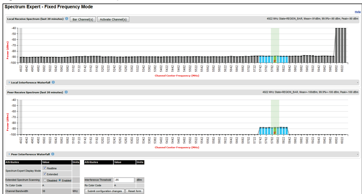
Figure 196 Spectrum Expert page for Fixed Frequency – Extended display mode
