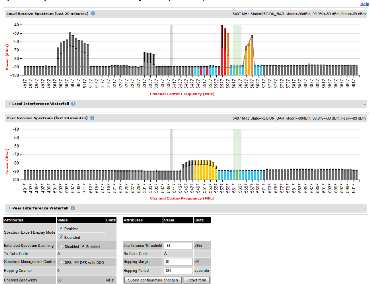
Figure 198 Spectrum Expert page with radar avoidance – Extended Display
