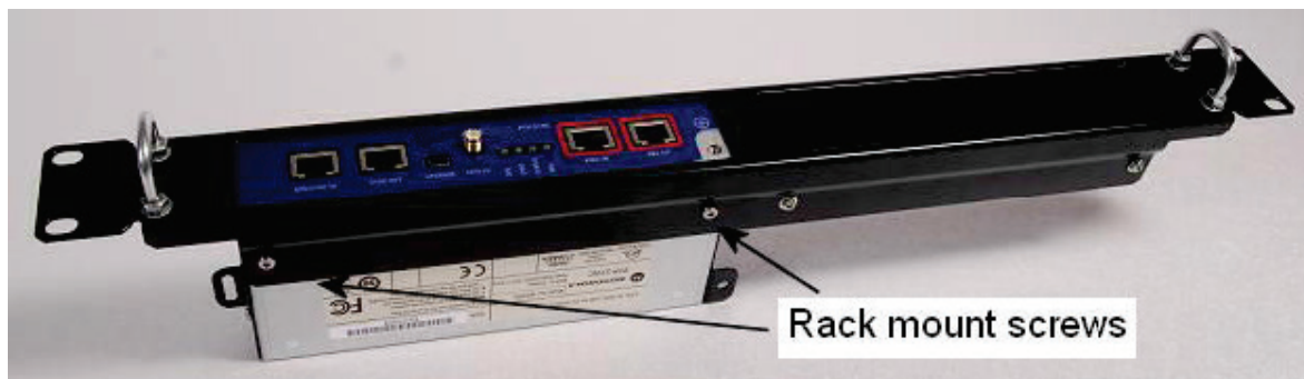
Figure 109 PTP-SYNC mounted in a rack
