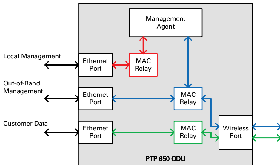
Figure 55 Ports and Services: Data + Out-Of-Band Management + Local Management
