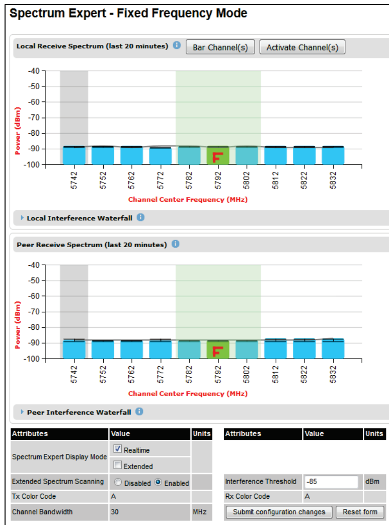
Figure 195 Spectrum Expert page for Fixed Frequency – Standard display mode
