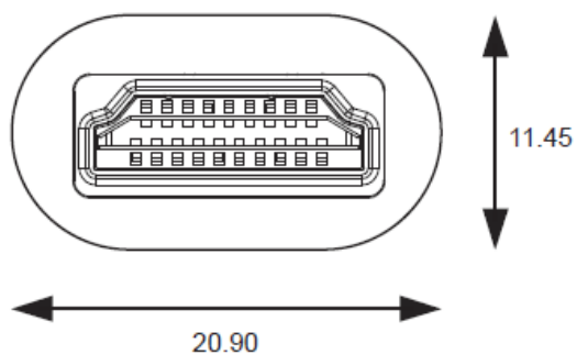
HDMI standard size (must not exceed)
