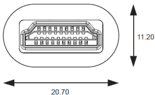
Locking HDMI size
