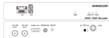
WiMi8520R Decoder
