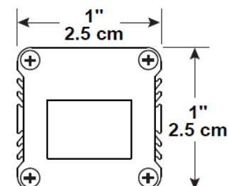
Left View
